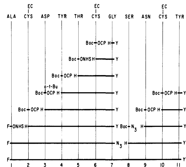
SYNTHESIS OF FRAGMENT A MOL. WT. 1,589
